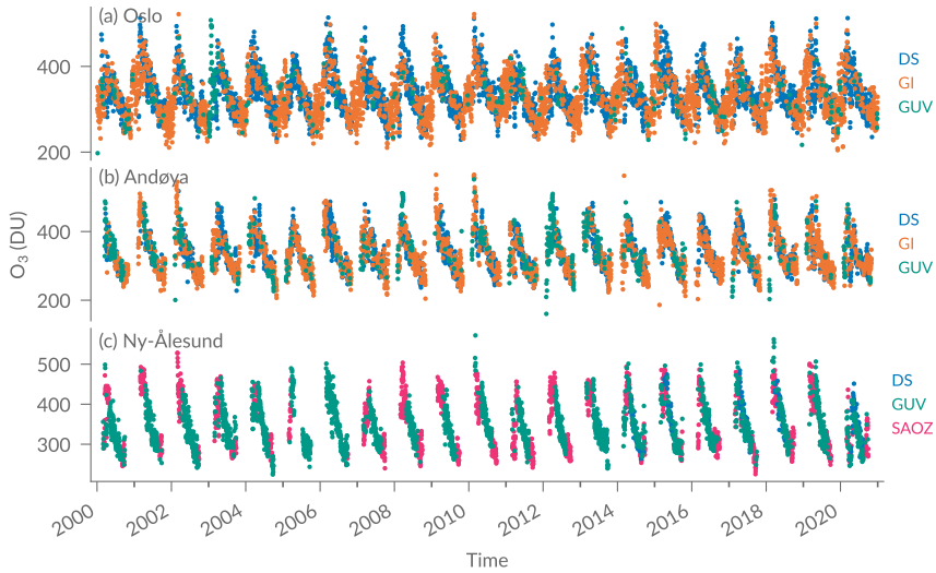
Combined total ozone time series from various ground-based measurements
