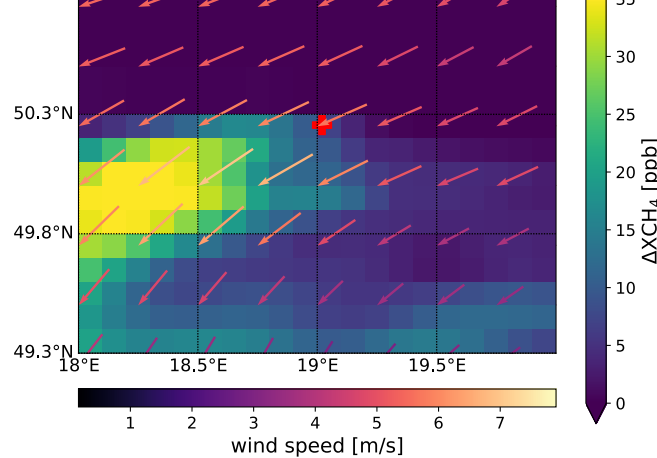
(b) CAMS forecast \Delta XCH_4 (bg=1829.1 ppb)
