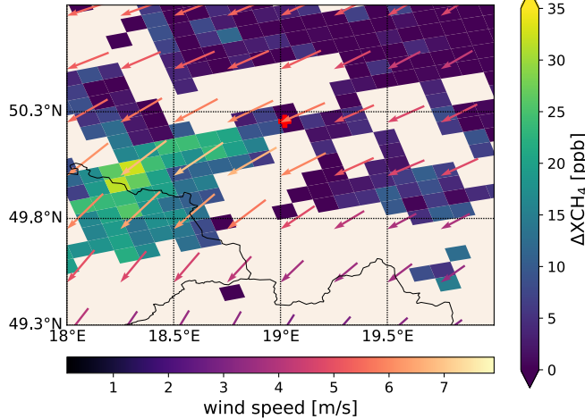
(a) TROPOMI \Delta XCH_4 (bg=1831.87 ppb)
