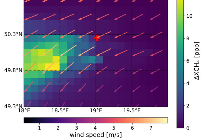
(c) Modelled \Delta XCH_4
